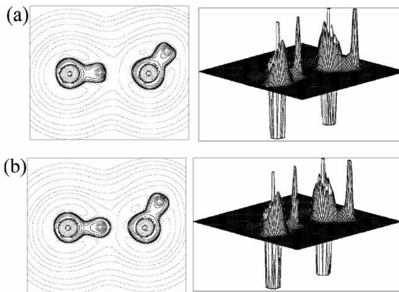
Figure 2. Contour plots and relief maps of \nabla^2\rho for the proton-transferred structure of (H_2O)_2^+ : (a) HF calculations and (b) DFT calculations using the B3LYP XC functional.
